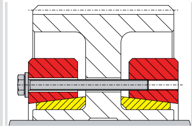
Shrink Disc Type SDG
