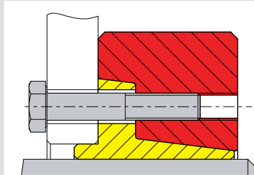
Locking Unit Type AS
